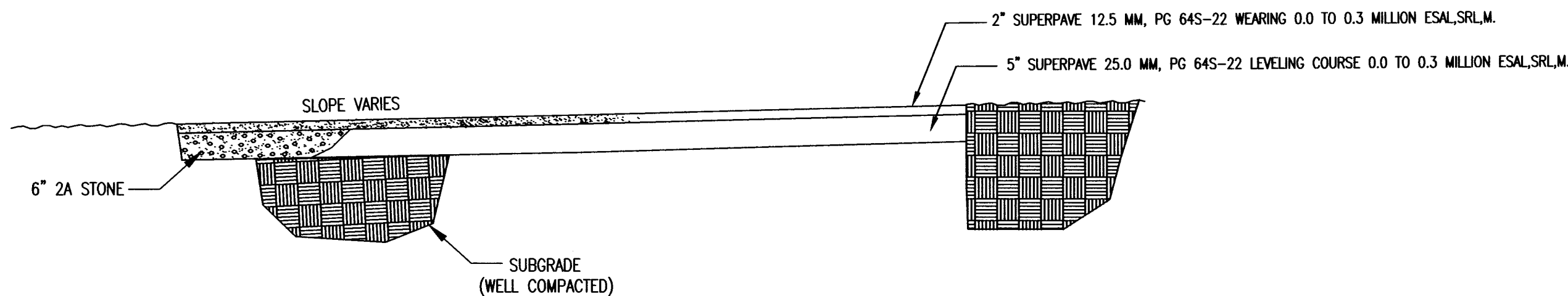
TYPICAL CROSS SECTION OF PROPOSED PARKING LOT ( NO SCALE )
